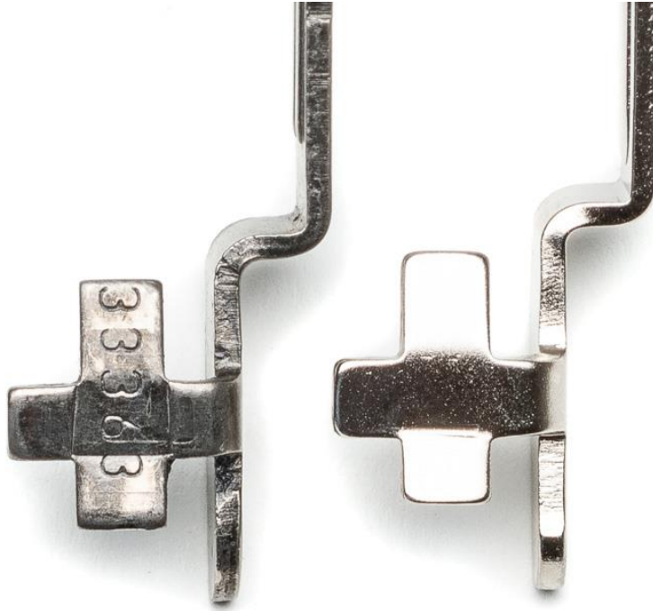
Glock Factory Trigger Bar
